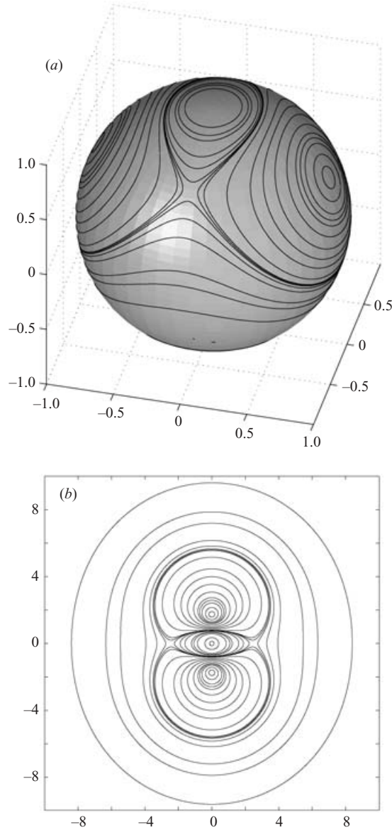
FIGURE 4. Solution for N = 2 , a = 1 and \theta_0 = \pi/3 shown in orthographic (a) and stereographic projection (b). The corresponding values of b and \Omega_{max} are 2.78 and -173.93 respectively. There are point vortices, each of circulation 2\pi , at both the north and south poles.
