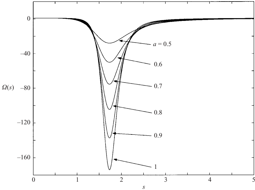
FIGURE 5. Graph of \Omega(s) against s for N=2 , \theta_0=\pi/3 and a=0.5, (0.1), 1 . The respective values of \Omega_{max} are -27.93, -50.09, -75.51, -104.55, -137.35 and -173.93 . As a increases, the vorticity profiles become more concentrated about the extremal value \Omega_{max} which itself increases in magnitude with increasing a .
