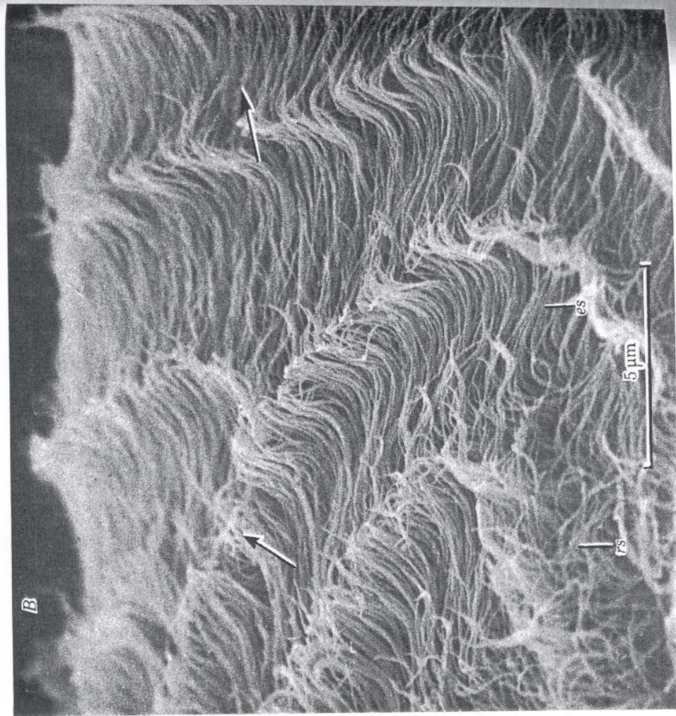
Figure 14 A scanning electron micrograph following rapid fixation of the ciliated protozoan Opalina (from Tamm & Horridge 1970). As in the preceding figure, the in vivo metachronal wave orientation is reflected in the pattern over the fixed specimen. Arrows indicate the directions of the metachronal wave. The key difference between the two specimens is that this figure is limited to all or part of a single cell. (We are indebted to Dr. S. L. Tamm for this photograph.)
