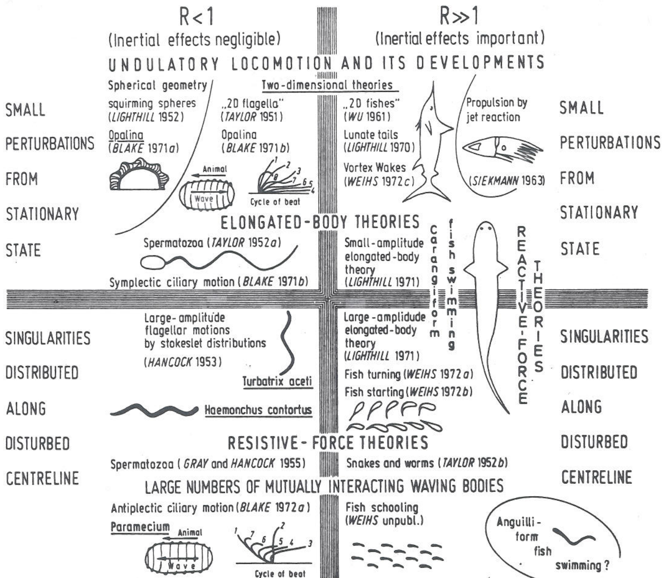
FIG. 1. Illustrating subdivisions of hydrodynamic theory relevant to aquatic animal locomotion.
