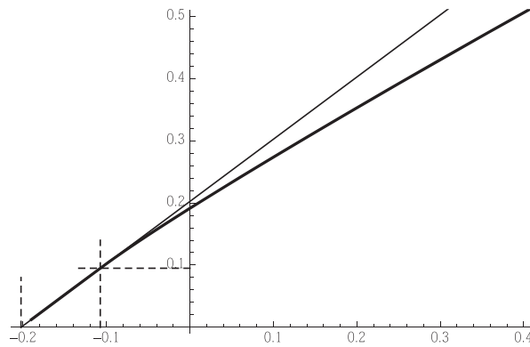
FIG. 1. The curve \alpha \mapsto \mu_{a,p}(\alpha) with p = 4 and a = 0.45 . The only solutions to (C1) are the constant functions for any \alpha such that -a^2 = -0.2025 \leq \alpha \leq -0.1075 and, in this range, \mu_{a,p}(\alpha) = a^2 + \alpha . A branch of non-constant optimizers of (2) bifurcates at \alpha = -0.1075 .
