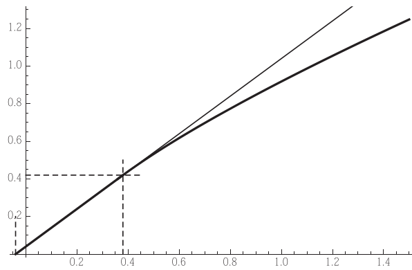
FIG. 2. The curve \alpha \mapsto \mu_{a,p}(\alpha) with p = 4 and a = 0.2 . Here the branch of non-constant optimizers of (2) bifurcates at \alpha = 0.38 which corresponds to a^2(p+2) + \alpha(p-2) = 1 .
