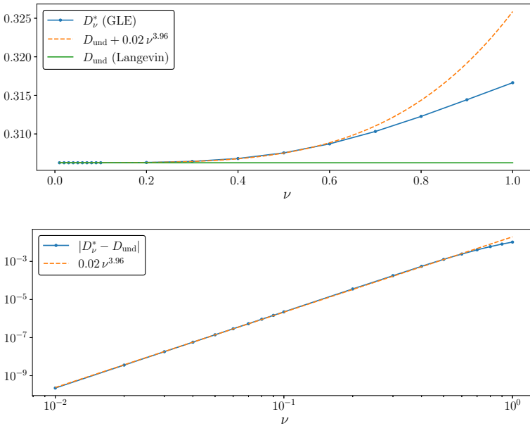
Fig. 6 Comparison between the effective diffusion coefficients (multiplied by \gamma ) for the Langevin and the generalized Langevin dynamics in the underdamped limit, in linear (top) and logarithmic (bottom) scales
