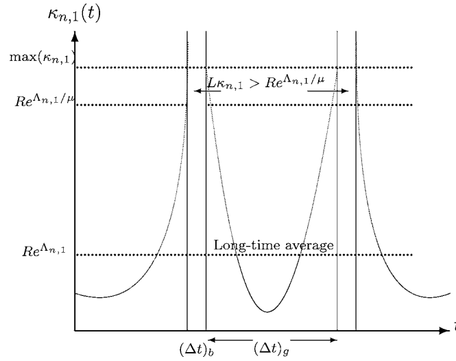
FIG. 1. A cartoon, not to scale, of good/bad intervals for some value of n \geq 3 .
